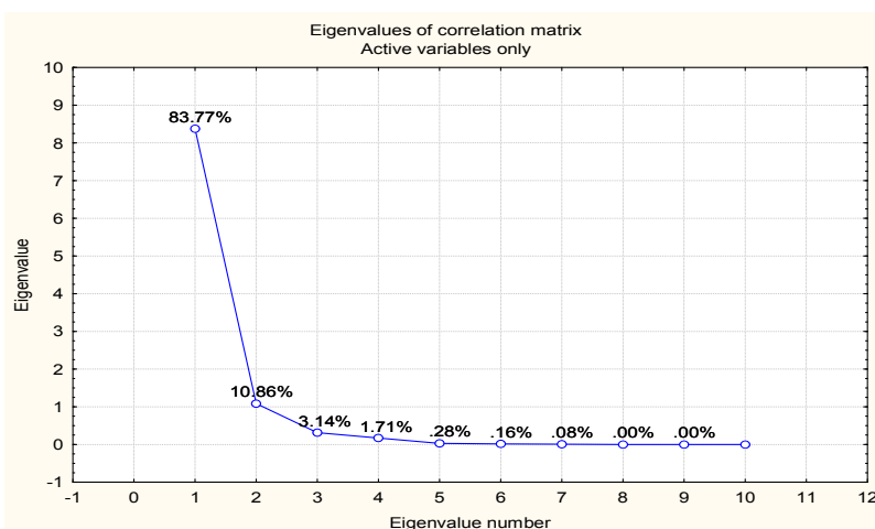
Fig. 1. Scree plot of the economic factors
