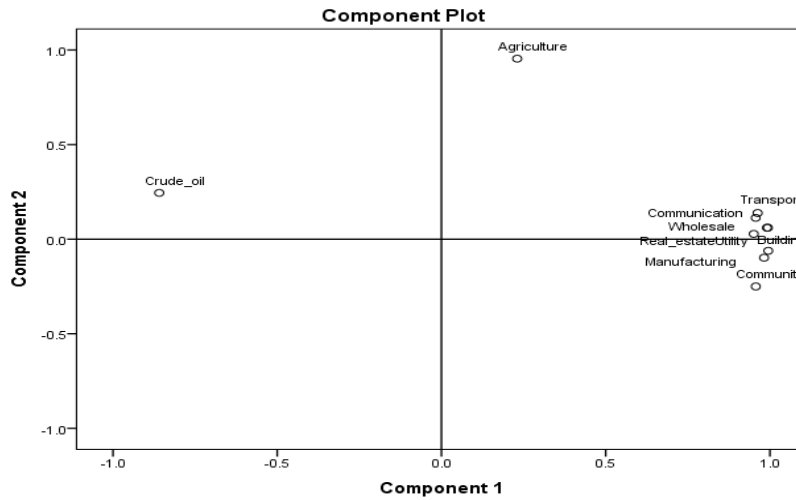
Fig. 2. Component plot of the economic factors
