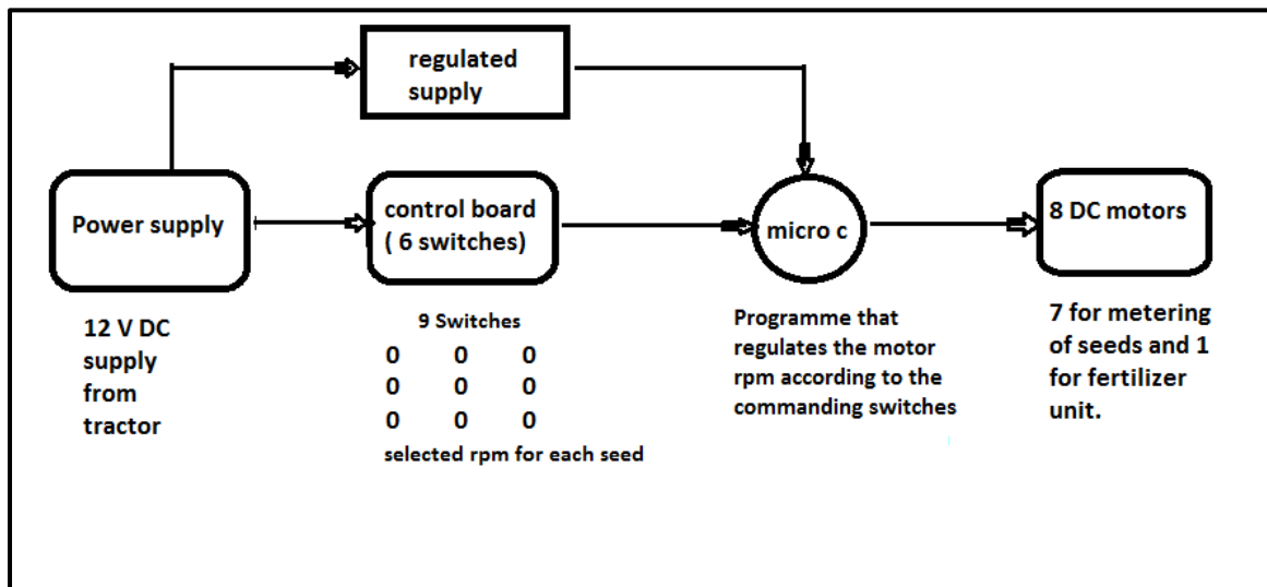
Fig. 1. Flow chart of the electronic seed metering mechanism
